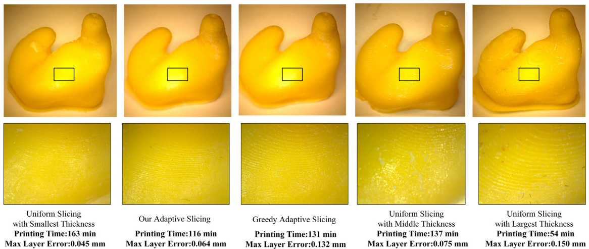
Fig. 10. Fabrication results of hearing aid model by different slicing methods.
