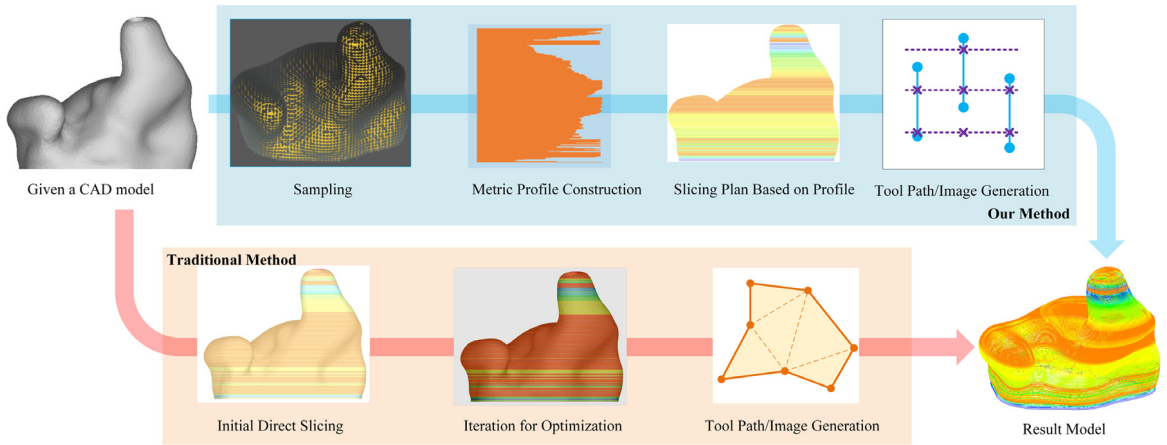
Fig. 2. Comparison between the traditional and our newly proposed adaptive slicing pipelines.
