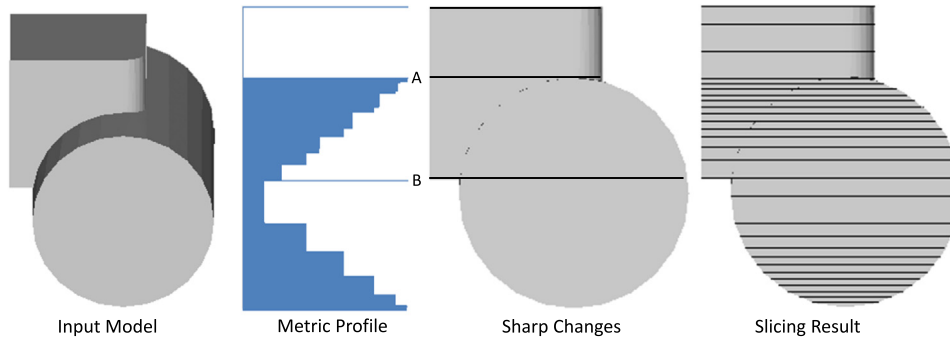
Fig. 4. Based on the metric profile of a given CAD model, sharp changes (located at A and B, which are the sharp transitions between the cube and the cylinder) can be detected. Our algorithm can successfully place slicing planes on these positions.
