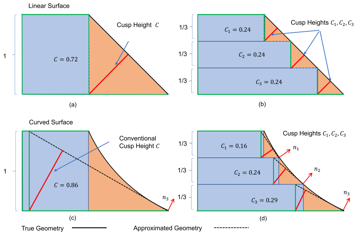
Fig. A.1. (a) and (c) illustrate the conventional method of approximating the printed geometry using cusp height; (b) and (d) are the proposed method for the approximation. The true geometry in the top row is a line, and the bottom row is a concave curve. The printed shapes are the extruded rectangles.
