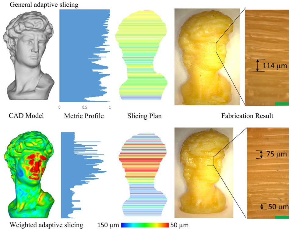
Fig. 7. Slicing comparison between weighted and non-weighted CAD model. The top part of the figure is a general slicing plan, which is almost uniform slicing, and the slicing in the bottom has small thicknesses in high weight positions. The colors in the slicing plan range from red to blue, indicating from the smallest thickness ( 50 \mu\text{m} ) to the largest thickness ( 150 \mu\text{m} ). The very right column shows the weighted result in bottom has smaller cusps, and the scale bar is 200 \mu\text{m} . (For interpretation of the references to color in this figure legend, the reader is referred to the web version of this article.)
