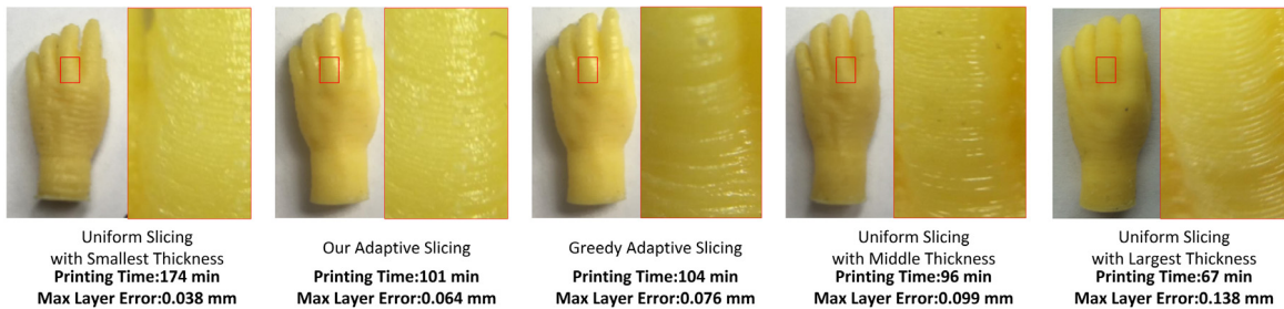
Fig. 11. Fabrication results of hand model by different slicing methods.
