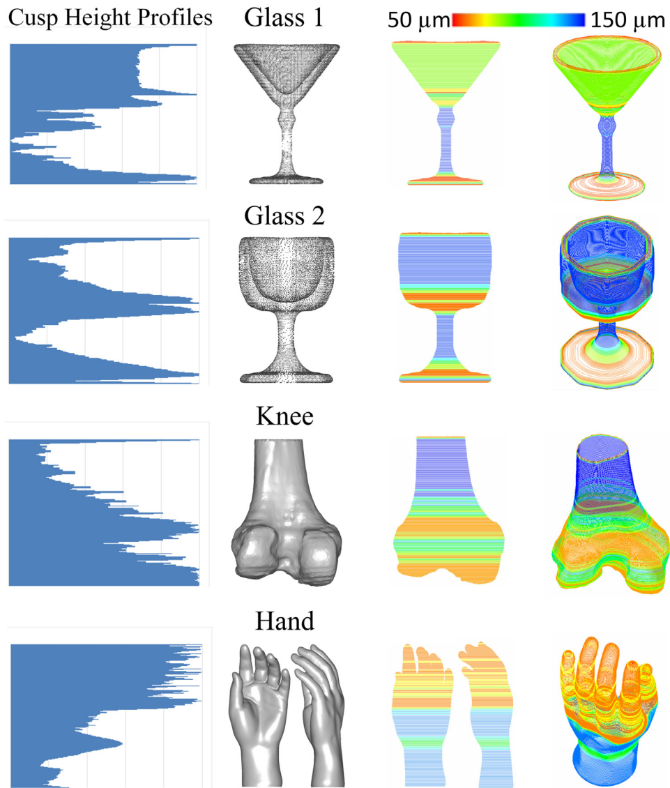
Fig. 9. Adaptive slicing results of various models.
