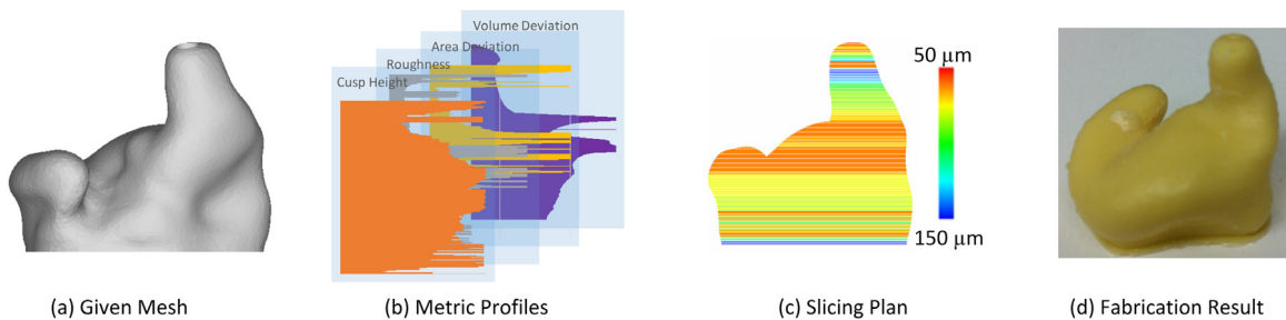
Fig. 1. Given a mesh model with weights on faces (a), the metric profiles (b) are extracted to describe the surface metric distributions along a building direction. Based on these profiles and the mesh weight, an optimal slicing plan (c) can be computed. The color scale in (c) represents the layer thickness value, and the smaller the layer thickness is, the color is closer to the red end. And all the figures in this paper share this same color scale for layer thickness. The result of the model fabricated by the optimal slicing is shown in (d), and the comparisons can be found in Fig. 10. (For interpretation of the references to color in this figure legend, the reader is referred to the web version of this article.)
