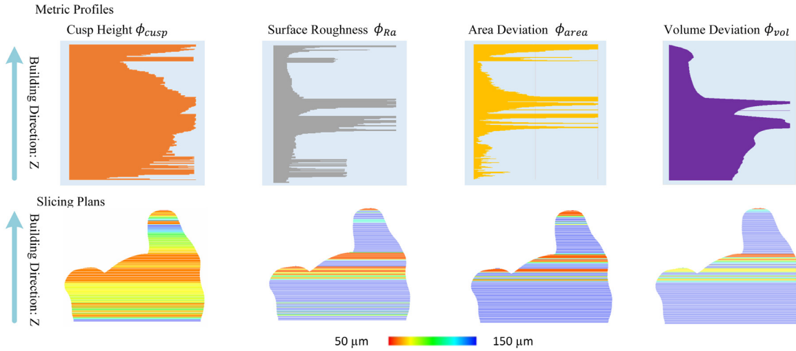
Fig. 5. Metric Profiles with different geometric error are shown in the top and the corresponding slicing plans are shown in the bottom. The colors in the slicing plan range from red to blue, indicating from the smallest thickness ( 50 \mu\text{m} ) to the largest thickness ( 150 \mu\text{m} ). (For interpretation of the references to color in this figure legend, the reader is referred to the web version of this article.)
